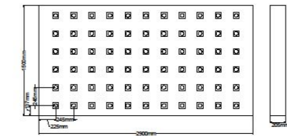
7-11 Gas Station double side lightbox (1) EZ-LED MAXI Number: 132 Pcs (66Pcs Each side) 12V DC/ 132W
