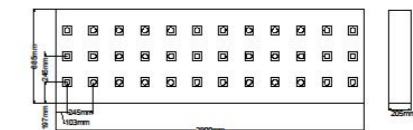
7-11 Gas Station double side lightbox (2) EZ-LED MAXI Number: 72Pcs (36Pcs Each side) 12V DC/ 72W
