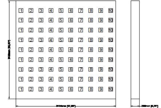
7-11 LOGO EZ LED MAXI Number: 180 Pcs (90 Each Side) 12V DC/180W
