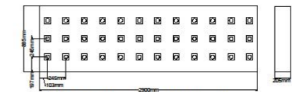
7-11 Gas Station double side lightbox (3) EZ-LED MAXI Number: 72Pcs (36Pcs Each side) 12V DC/ 72W
