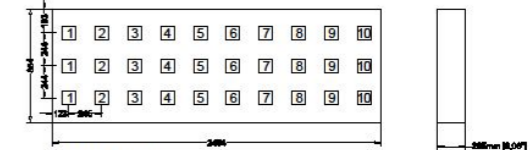
7-11 24 Hour EZ LED MAXI Number: 60 Pcs (30 Each Side) 12V DC/60W
